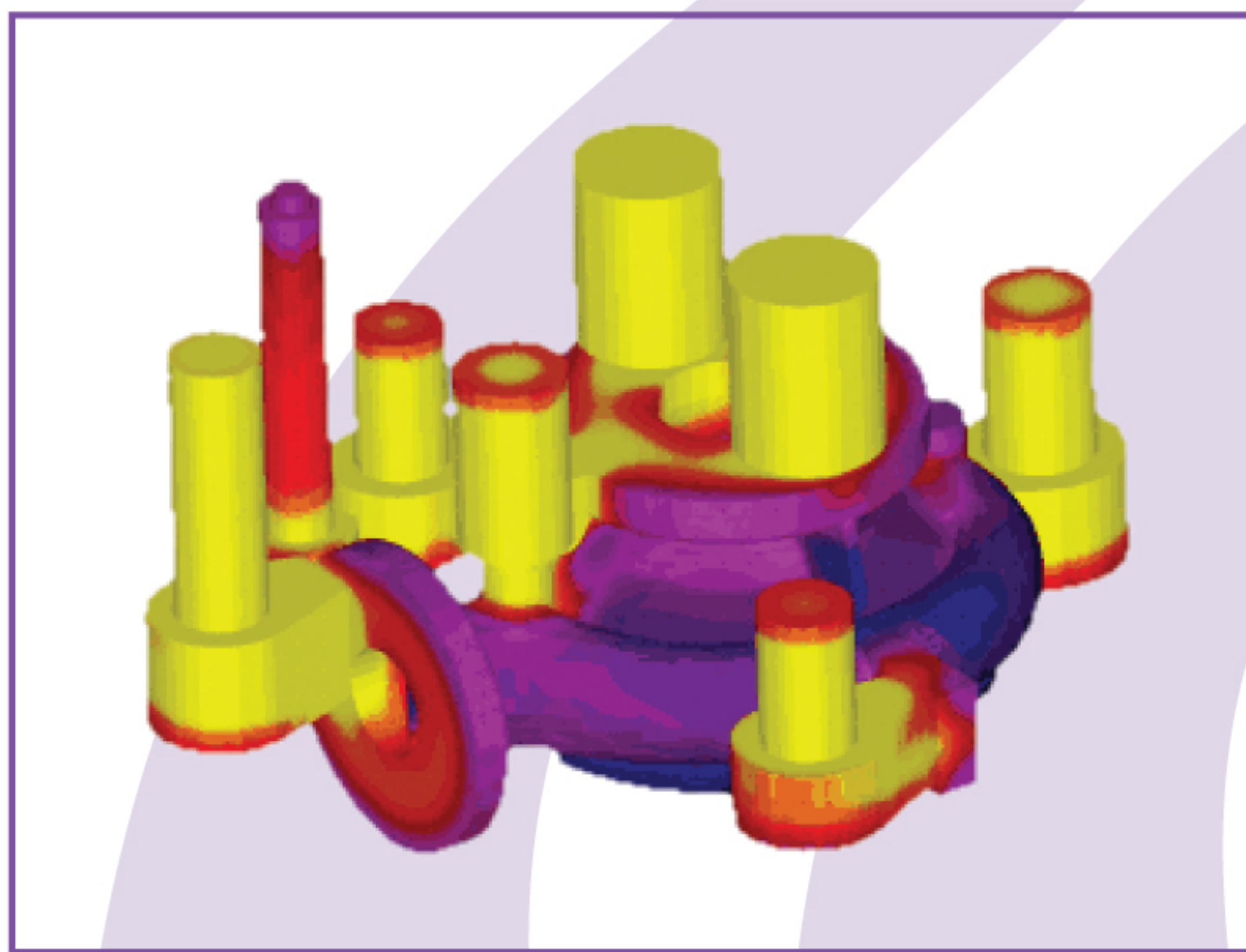
CASTING SIMULATION
